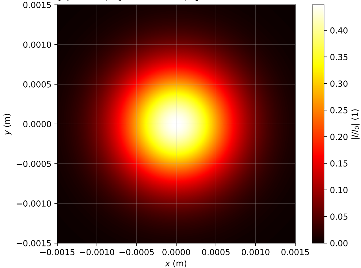
Intensity profile I(x, y, z = 2.866m)/I_0 , \text{Pin}=0.3\text{Pcr} , artificial time
